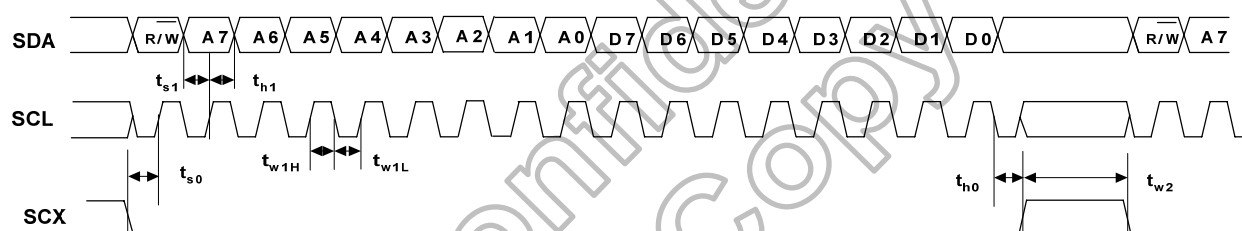
Figure 8.1: Serial Interface Signal Timing Chart
