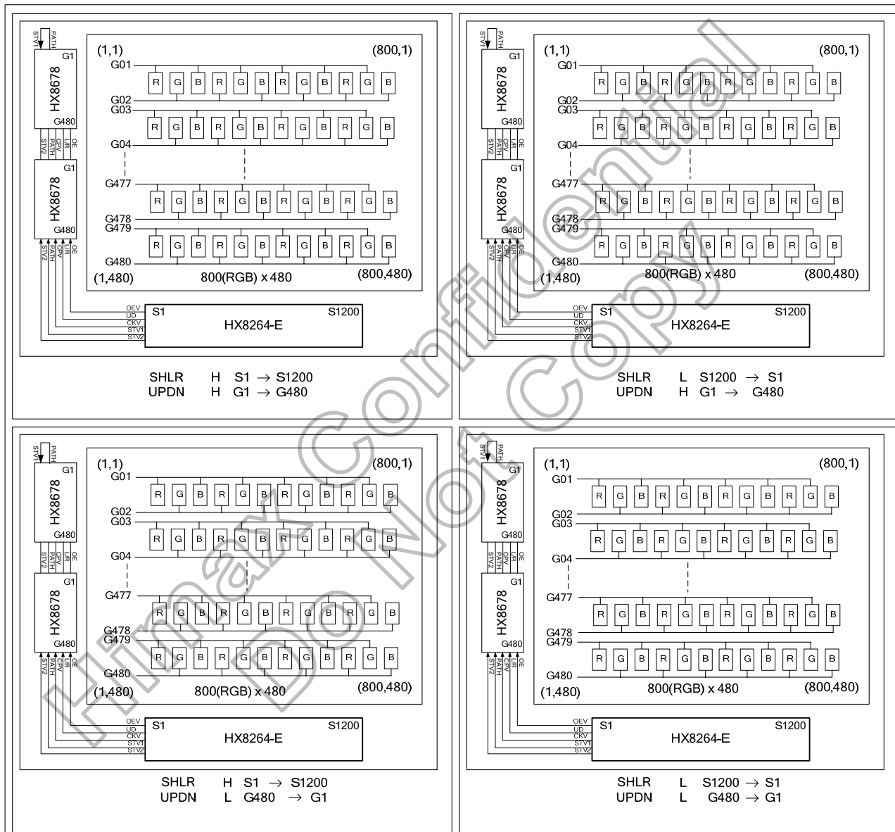
Figure 3.2: HX8264-E dual gate 800(RGB) x 480 application block diagram
