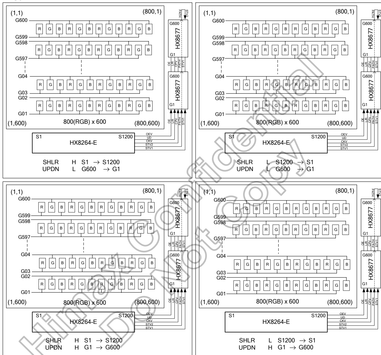
Figure 3.5: HX8264-E dual gate 800(RGB) x 600 application block diagram
