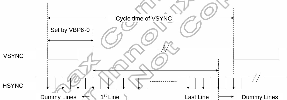
Figure 7. 16 No. of Clock Cycle of HSYNC
