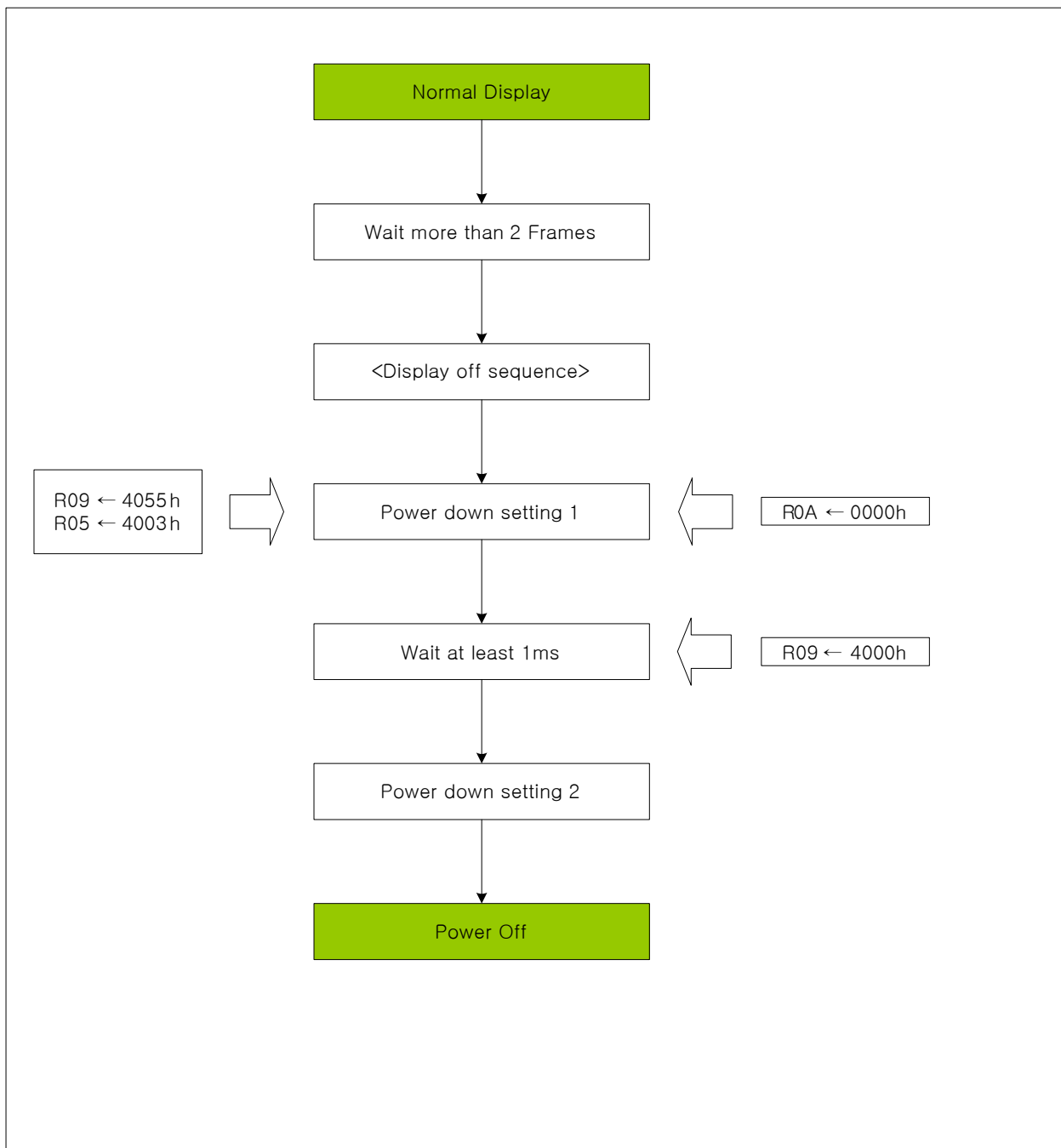
Figure 7. 33 Power Down Sequence when SPSW connect to VSS (CPE = VSS)
