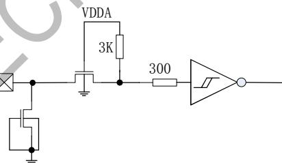
Figure 3-2 Reset Input Port Circuits
